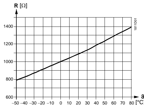
Characteristic LG-Ni 1000
