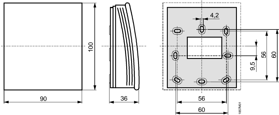
Drilling plan
